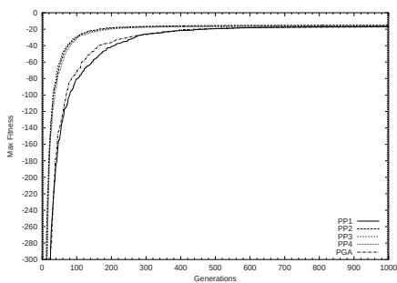
Fig. 4. Simulation (PP in Rosenbrock)
