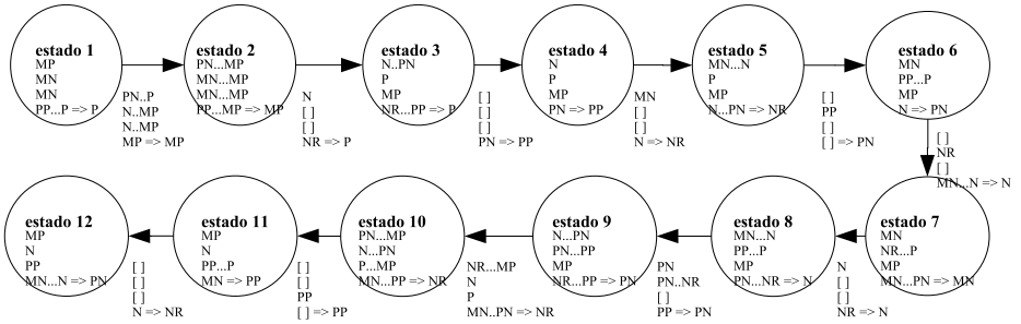
Fig. 5. Temporal Fuzzy Chain 1
