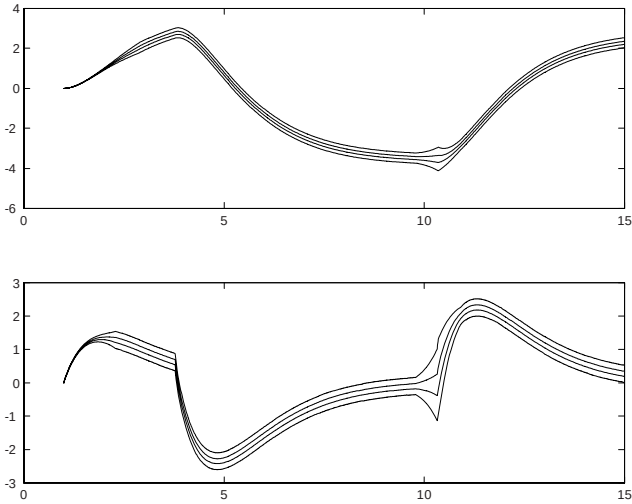
Fig. 4. Solution with the assumption that small velocity implies increasing uncertainty, second experiment
