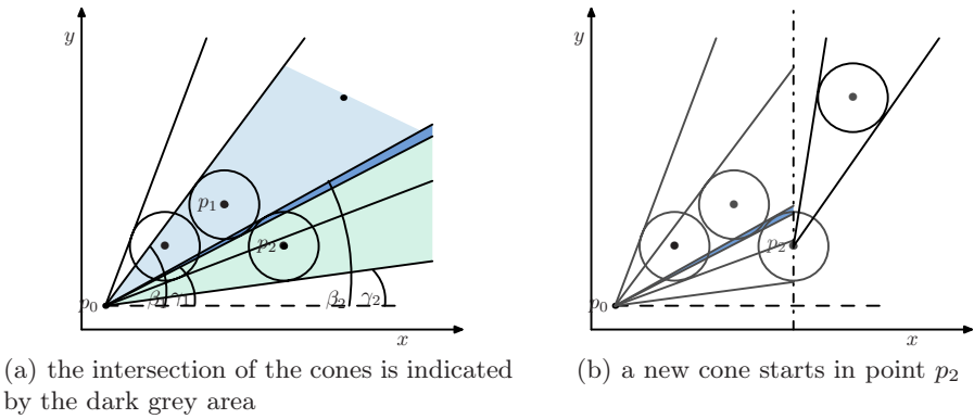
Fig. 1. An illustration of the algorithm for the uniform \varepsilon -approximation
