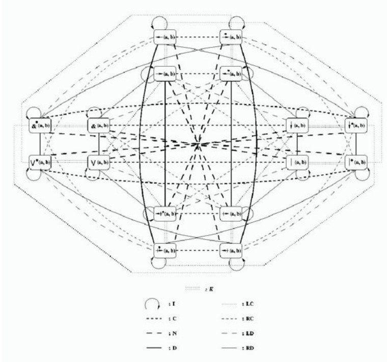
Fig. 1. Graph of Group Transformations for Interval System m_3
