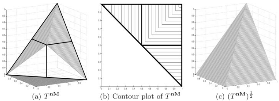
Fig. 3. Decomposition of the nilpotent minimum T^{\text{nM}}
