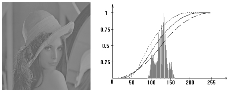
Fig. 4. Image "Lena" with very bad contrast (on the left) and histogram with determined membership functions (on the right). Significance of lines: as in the Fig. 2.
