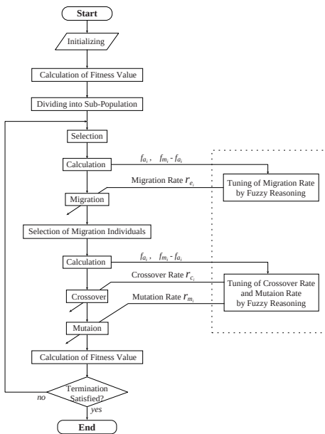
Fig. 1. Algorithm Flow of FASPGA
