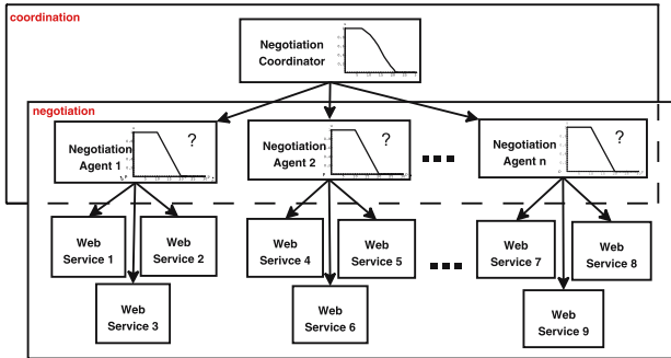
Fig. 2. Example of composition pattern with the aggregation of attribute values
