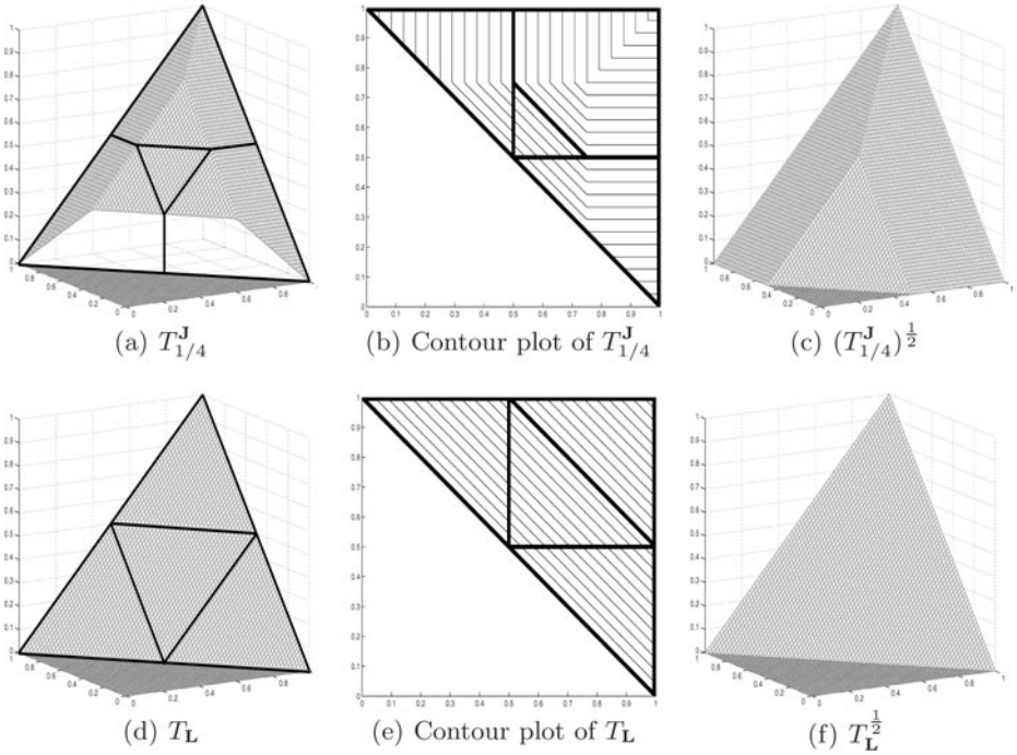
Fig. 4. Decomposition of the Jenei t-norm T_{1/4}^J and the Łukasiewicz t-norm T_L
