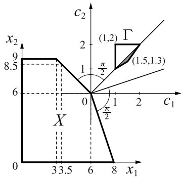
Fig. 3. Solution (6, 6)^T in Example 3
