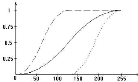
Fig. 1. Different shapes of S-function depend on a , b and c parameters. Lines denoting parameters: dashed line a = 0, b = 63.5, c = 127.5 ; solid line a = 0, b = 127.5, c = 255 ; dotted line a = 127.5, b = 191, c = 255
