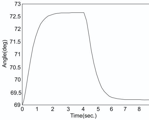
Fig. 5. Transient Response of of axis 2 using the proposed fuzzy controller
