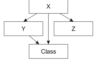
Fig. 3. A possibilistic network example
