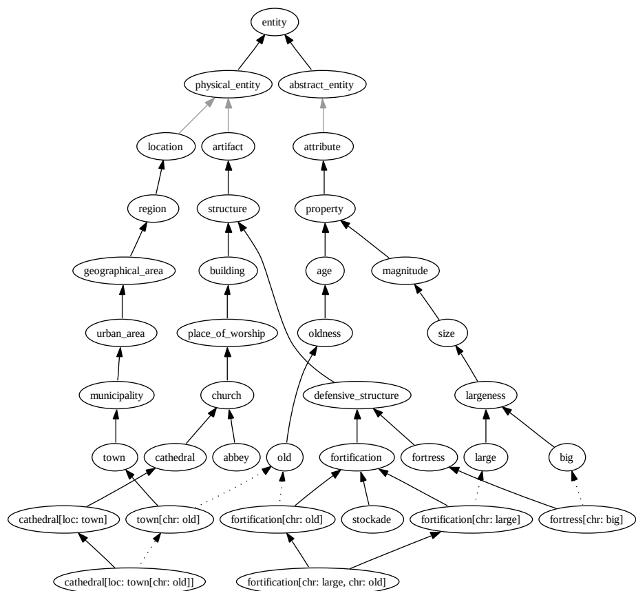
Fig. 1. An instantiated ontology based on a Wordnet ontology and the set of instantiated concepts \{cathedral[LOC: town[CHR: old]], abbey, fortification[CHR: large, CHR: old], stockade\}
