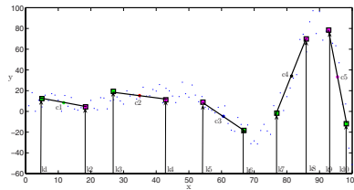
Fig. 1. Five local linear models using G-K algorithm
