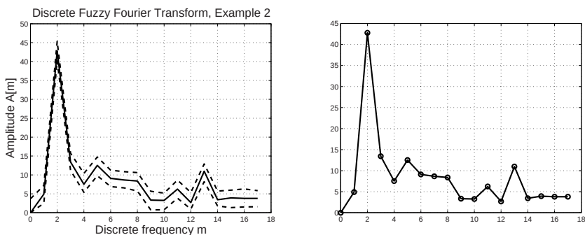
Fig. 3. Example 2. Discrete fuzzy Fourier transform (left). Solid line shows X_1[m] where \alpha = 1 , dashed lines show X_0^-[m] and X_0^+[m] for \alpha = 0 . Comparison of X_1[m] and conventional FFT (right), X_1[m] - solid line, FFT - points.
