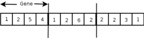
Fig. 1. Chromosome Structure
