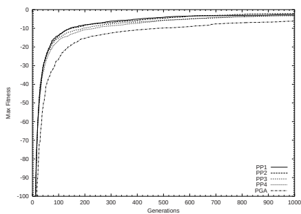
Fig. 3. Simulation (PP in Rastrigin)
