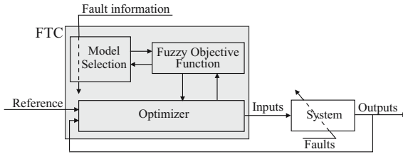
Fig. 2. FTC structure
