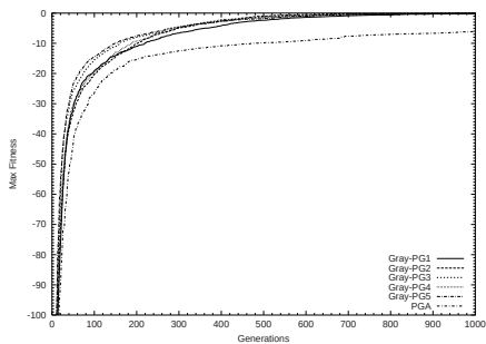
Fig. 7. Simulation (Gray-PG in Rastrigin)
