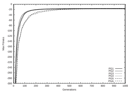
Fig. 6. Simulation (PG in Rosenbrock)
