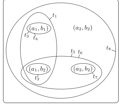
Fig. 1. The contexts induced by table 1
