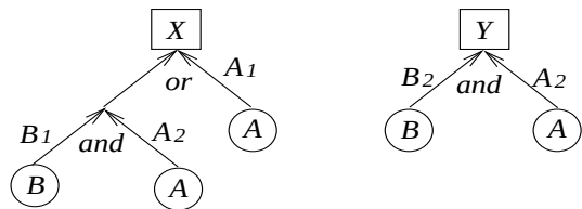
Fig. 1. Two example pattern trees
