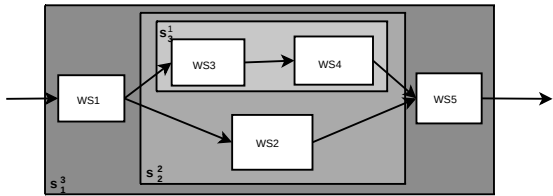
Fig. 1. Example of a composition pattern
