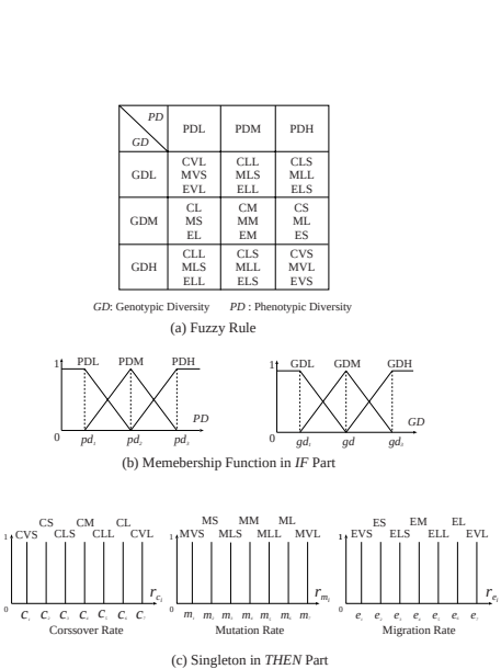
Fig. 2. Fuzzy Reasoning of DM-FASPGA
